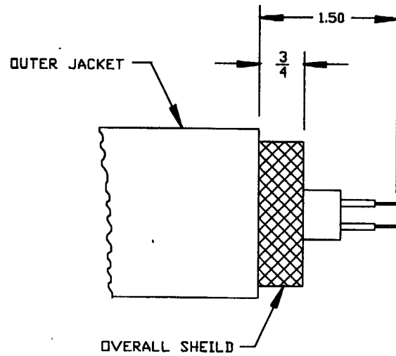
14 16 CABLE PREPARATION
