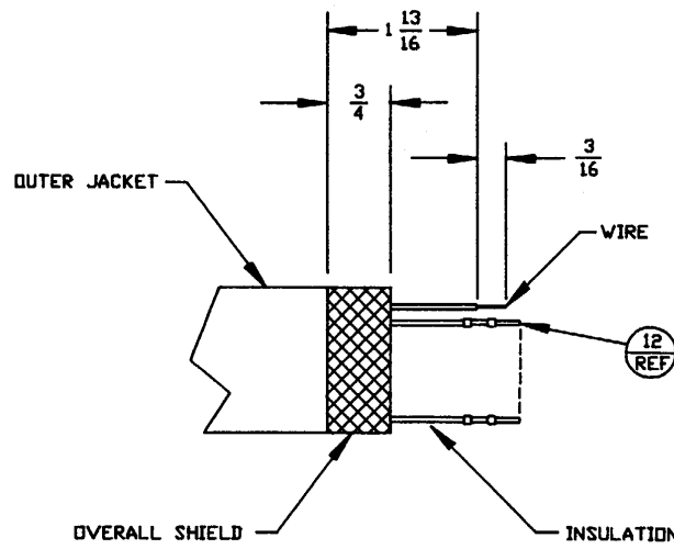
△14 CABLE PREPARATION
