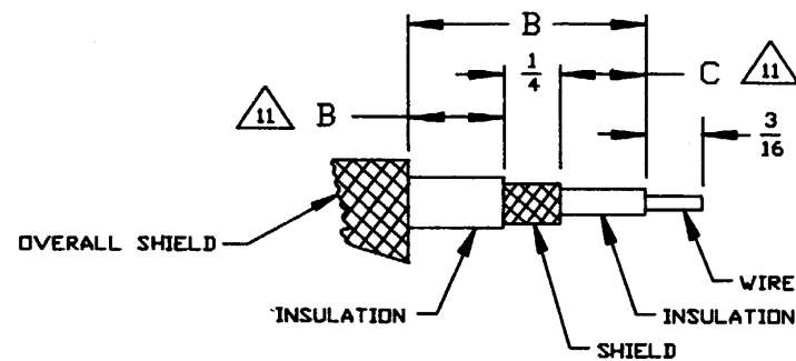
▲19 CABLE PREPARATION
