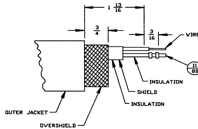
14 20 CABLE PREPARATION
