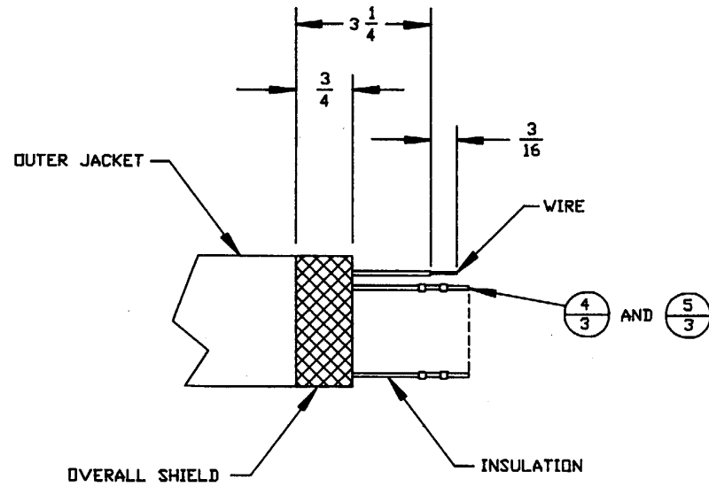
CABLE PREPARATION 15
