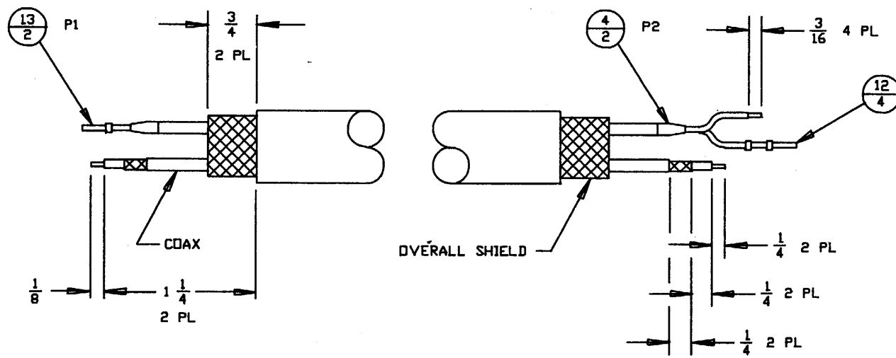
14 CABLE PREPARATION
