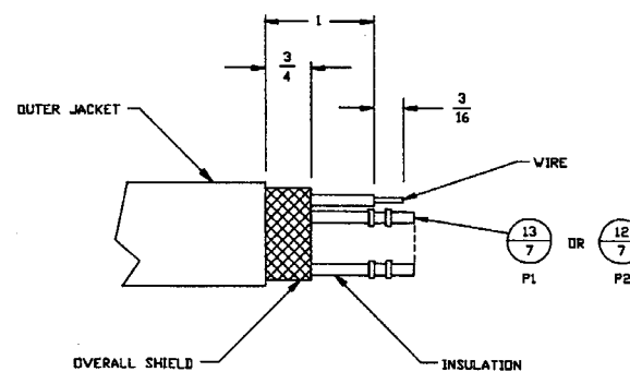
CABLE PREPARATION
