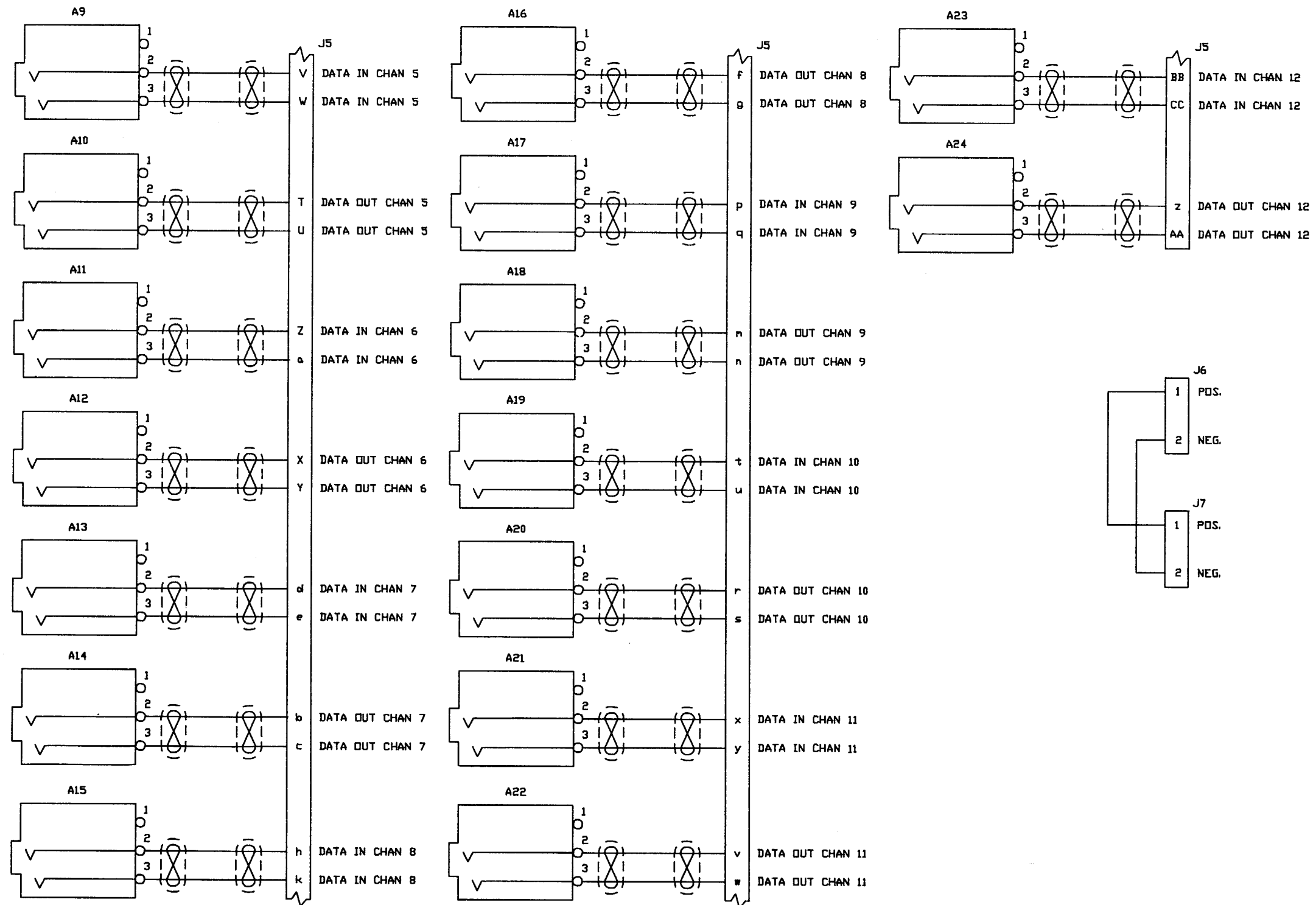
Schematic Diagram, Black Patch Panel, OPN (Sheet 2 of 2)
