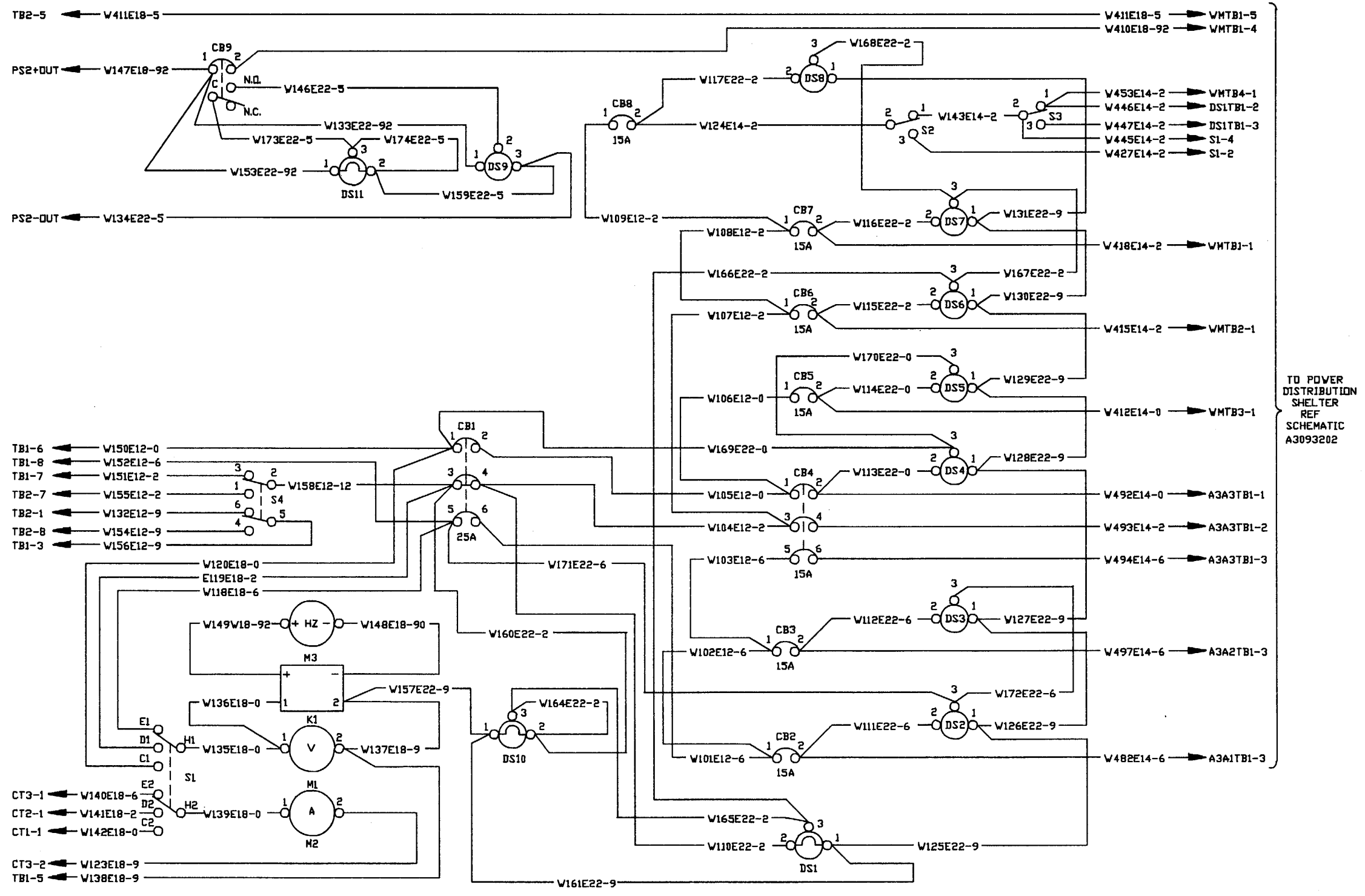
Schematic Diagram, Power Distribution Panel (Sheet 2 of 2)
