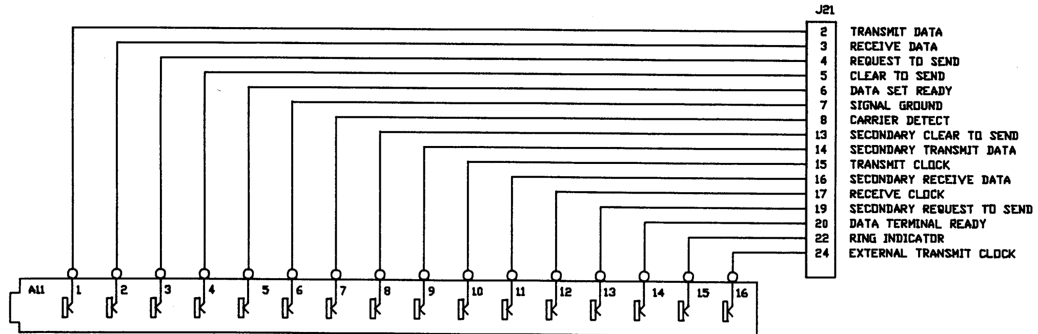
Schematic Diagram, Patch Panel - Red (Sheet 10 of 22)
