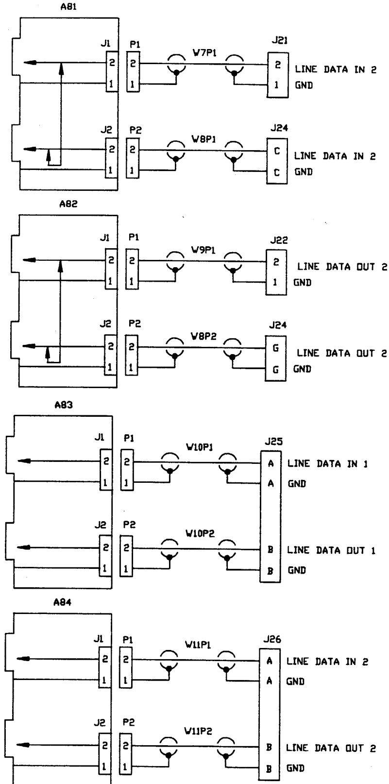
Schematic Diagram, Black Patch Panel - ANITY-30 (Sheet 6 of 6)
