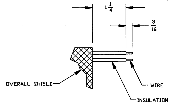
CABLE PREPARATION
