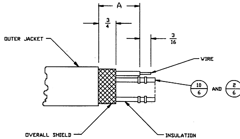
CABLE PREPARATION
