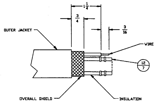
CABLE PREPARATION
