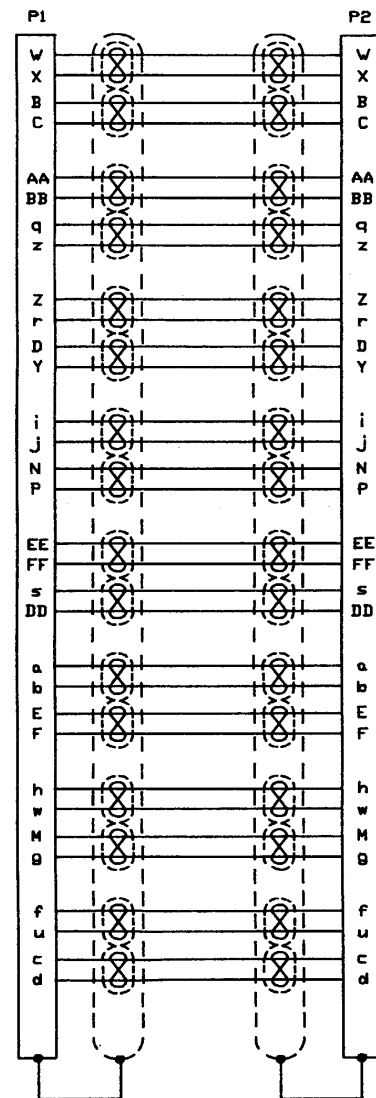
WIRING DIAGRAM
