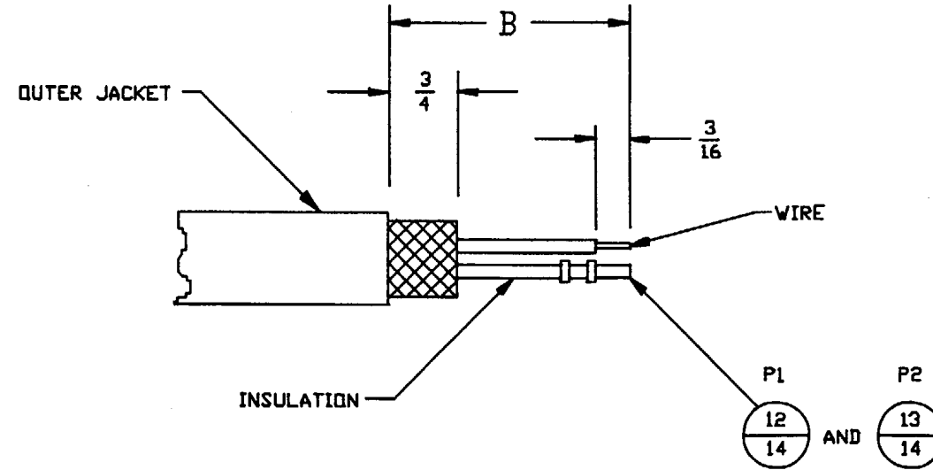
CABLE PREPARATION 13
