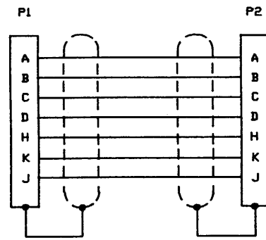
WIRING DIAGRAM
