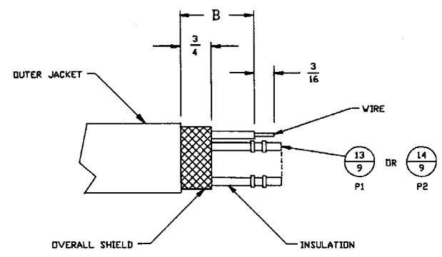
CABLE PREPARATION \triangle 15
