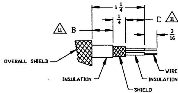
△19 CABLE PREPARATION
