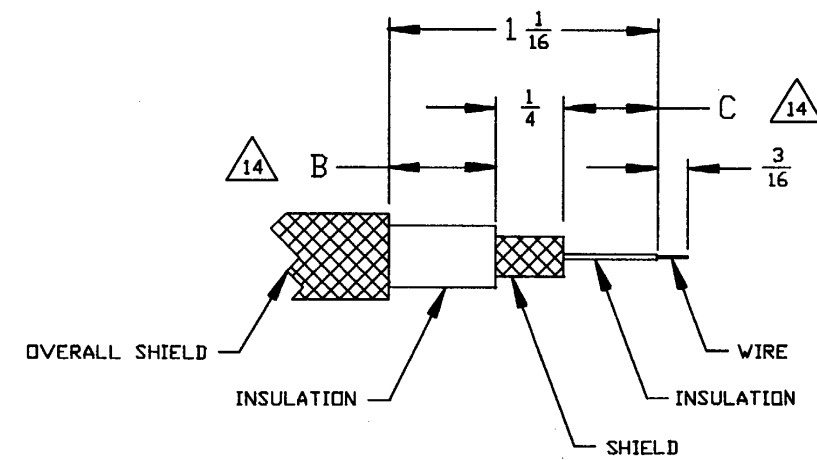
17 CABLE PREPARATION
