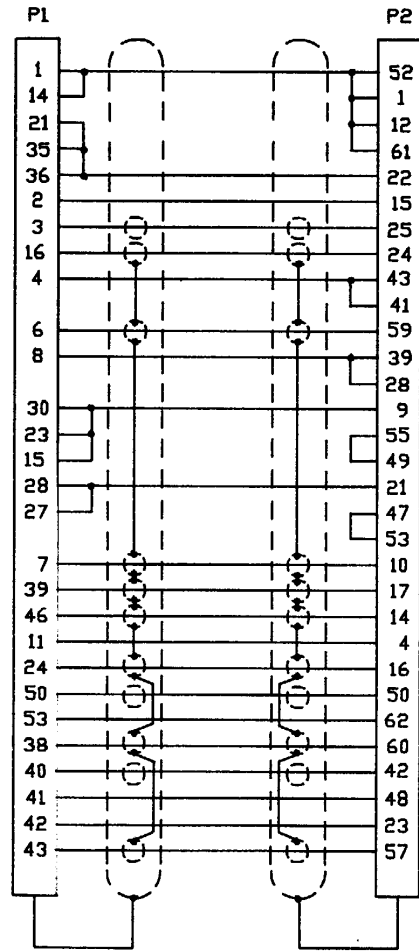
WIRING DIAGRAM
