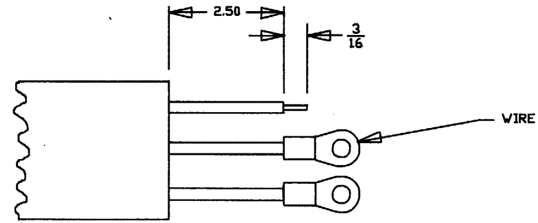
CABLE PREPARATION
