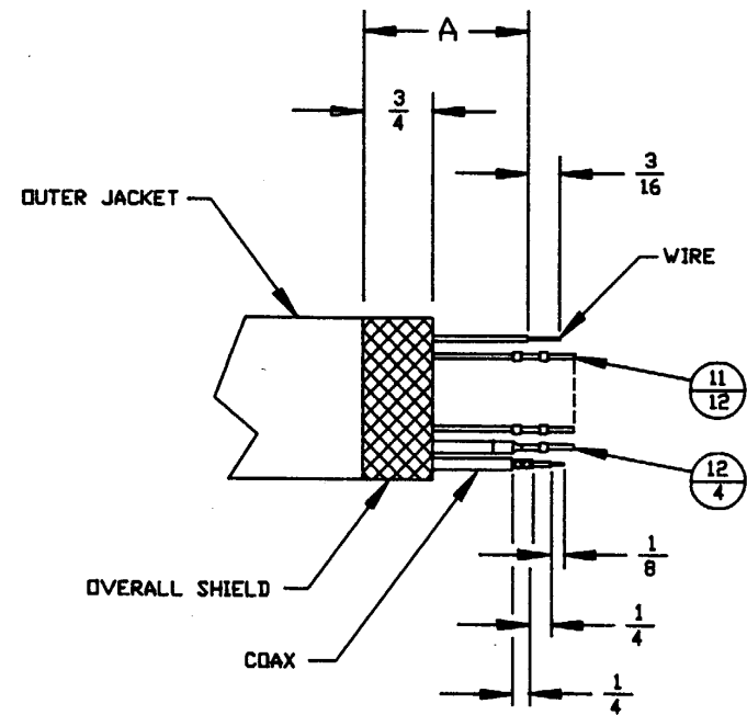
14 CABLE PREPARATION
