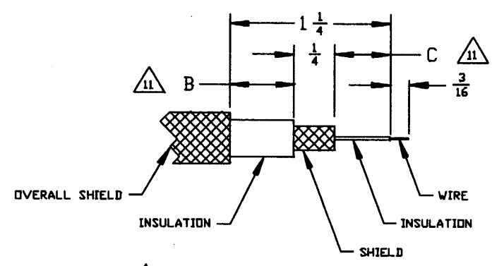
\Delta 18 CABLE PREPARATION
